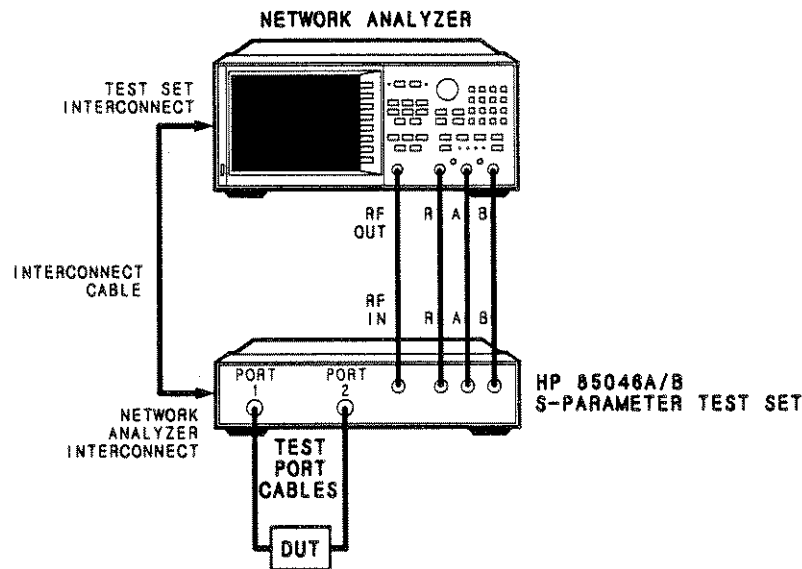
Figure 3-3. Typical Measurement Setup
