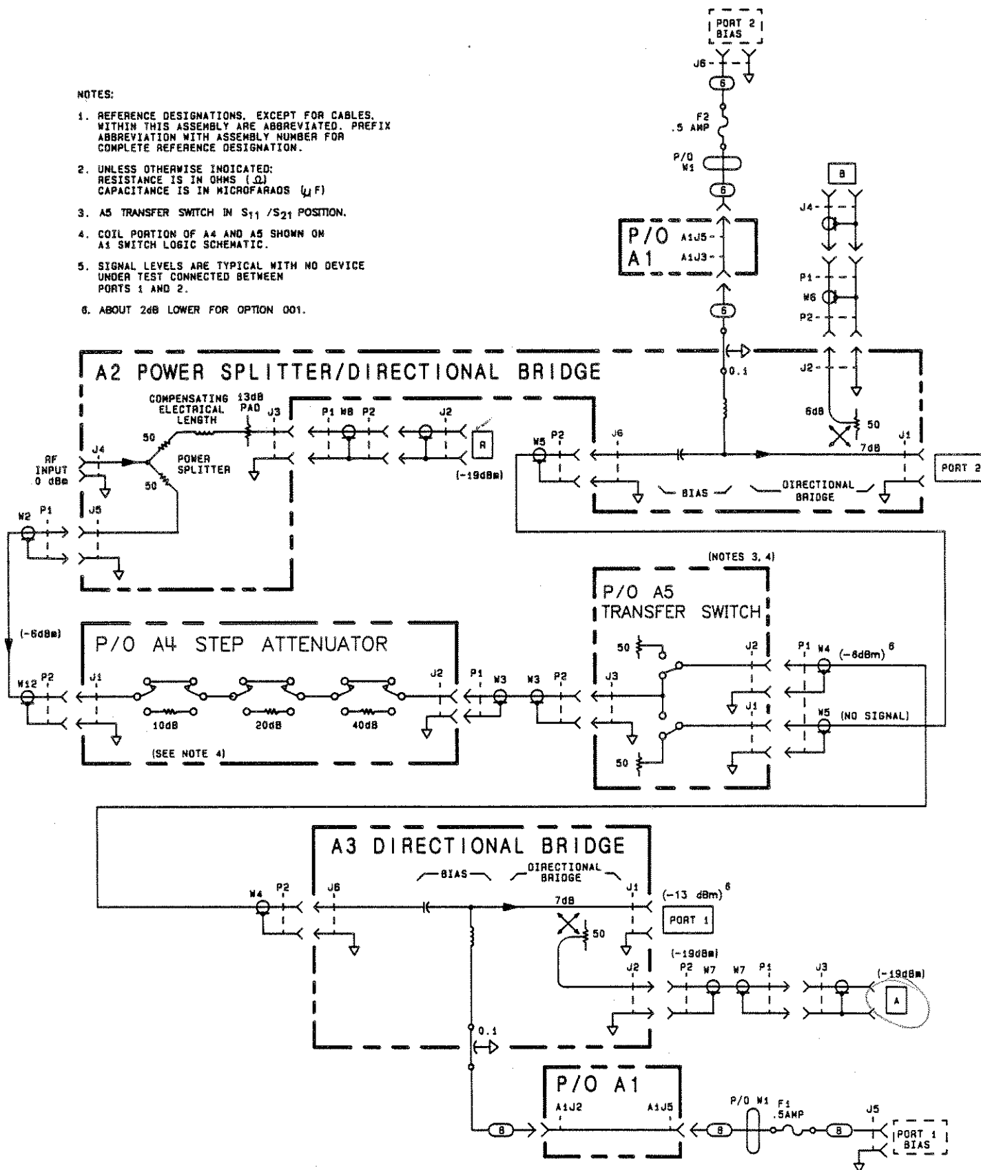
Figure 8-3. Schematic Diagram
