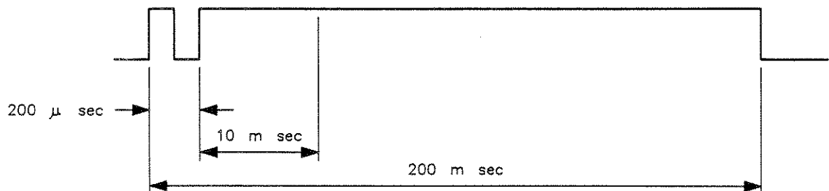
Figure 8-1. Test Set Interconnect Signal Lines and Sweep Delay Pulse
