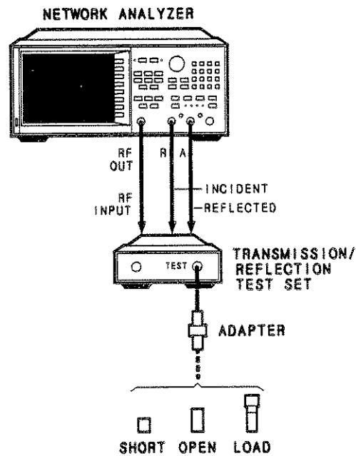
Figure 4-2. HP 85044A Calibration Set-up
