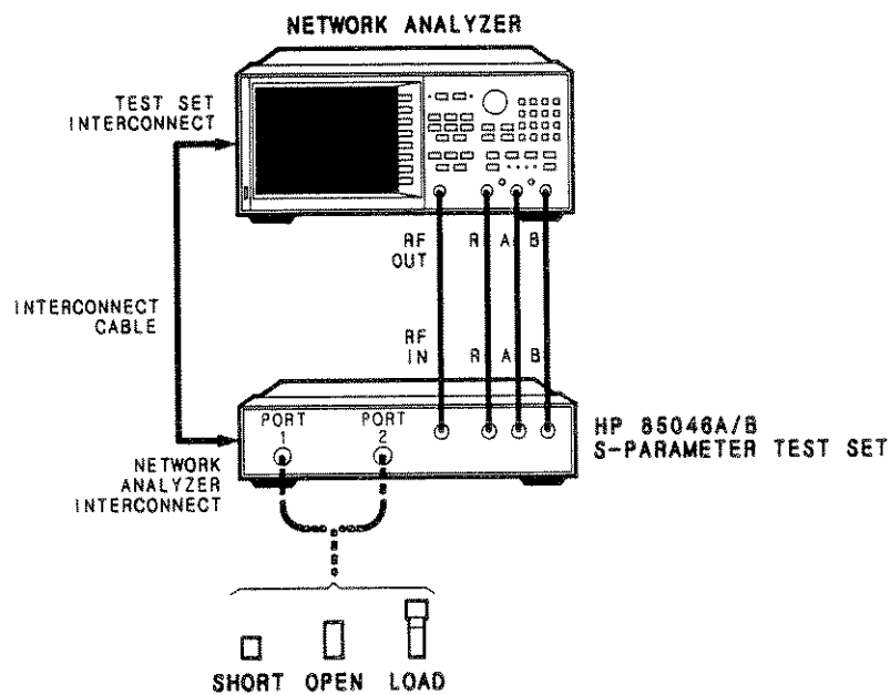
Figure 4-5. Source Match Test Setup
