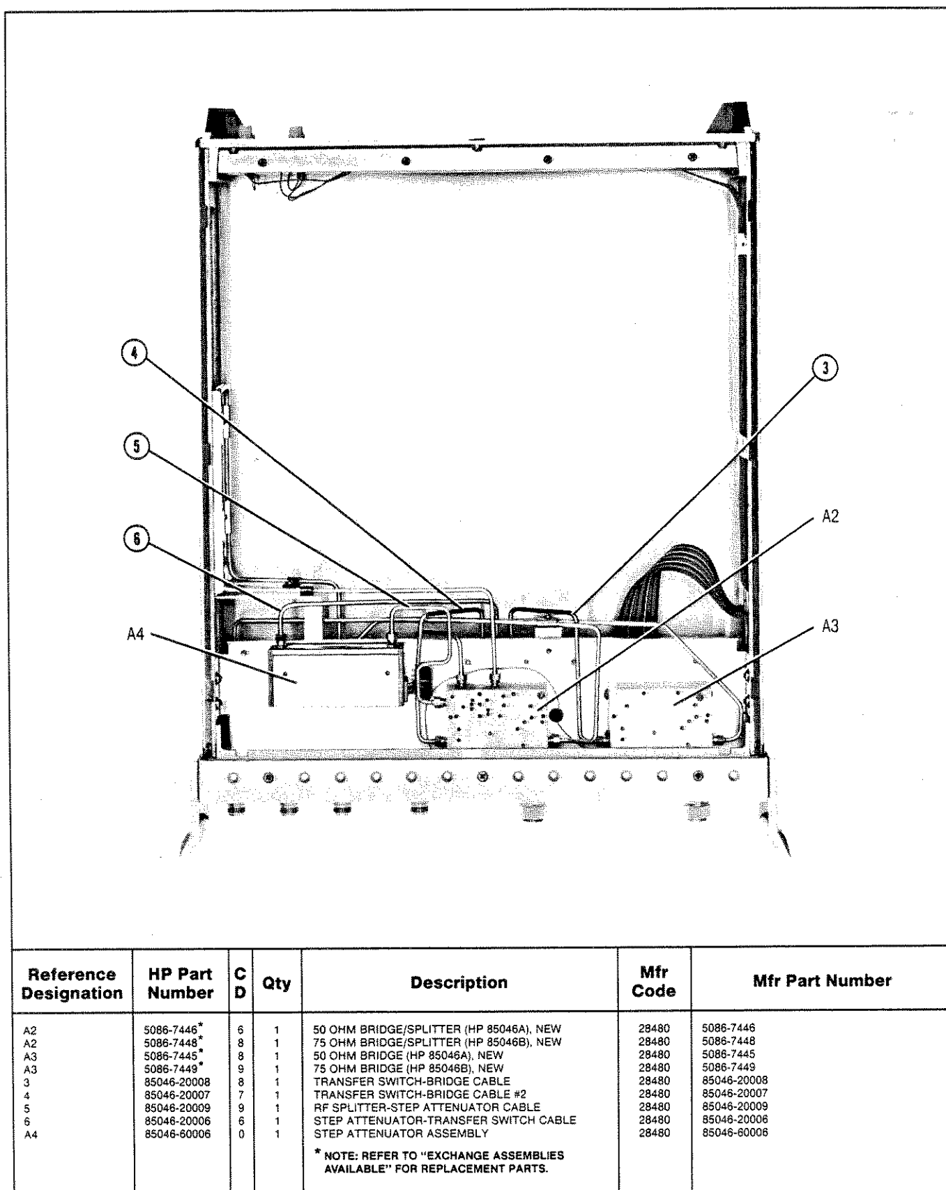
Figure 6-2 (2 of 2). Cables and Major Assemblies (bottom view)
