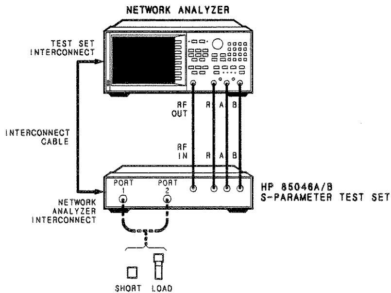
Figure 4-1. Directivity Test Setup
