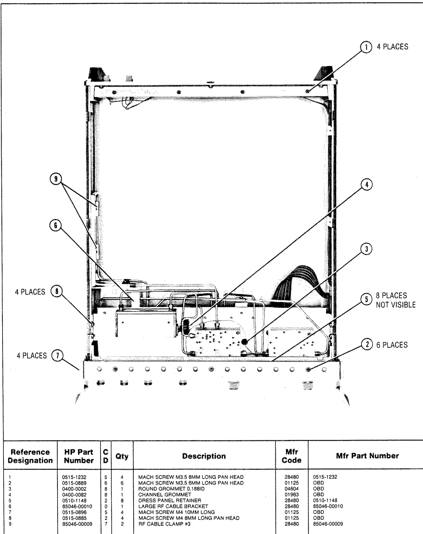
Figure 6-3 (3 of 4). Miscellaneous Parts (bottom view)
