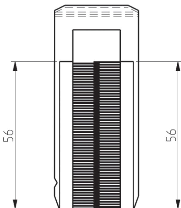
Anti-static brushes / Balais antistatiques Ref. 070100829A
