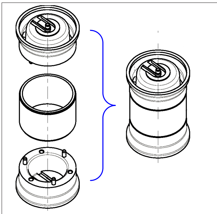
120-film Roller / Diabolo 120 Ref. 070100076A
