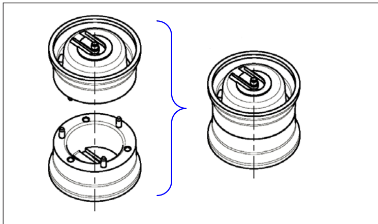
135-film Roller / Diabolo 135 Ref. 070100075A
