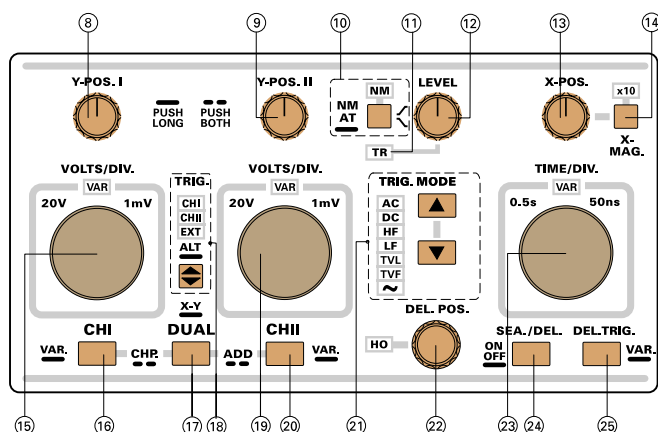
(25) DEL. TRIG. - VAR. - pushbutton with two functions.
